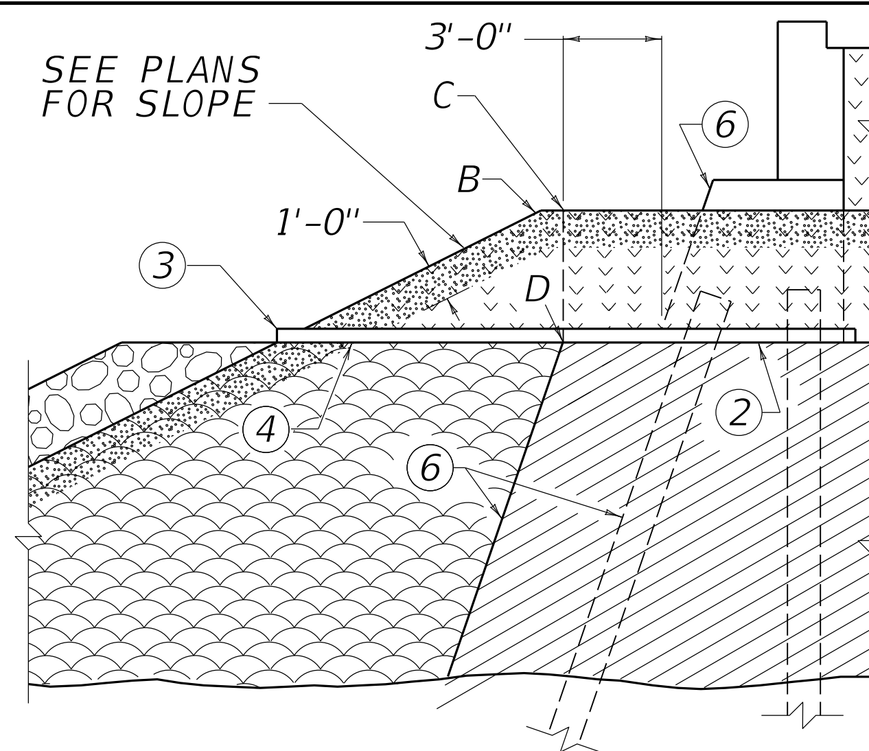
SECTION C-C
